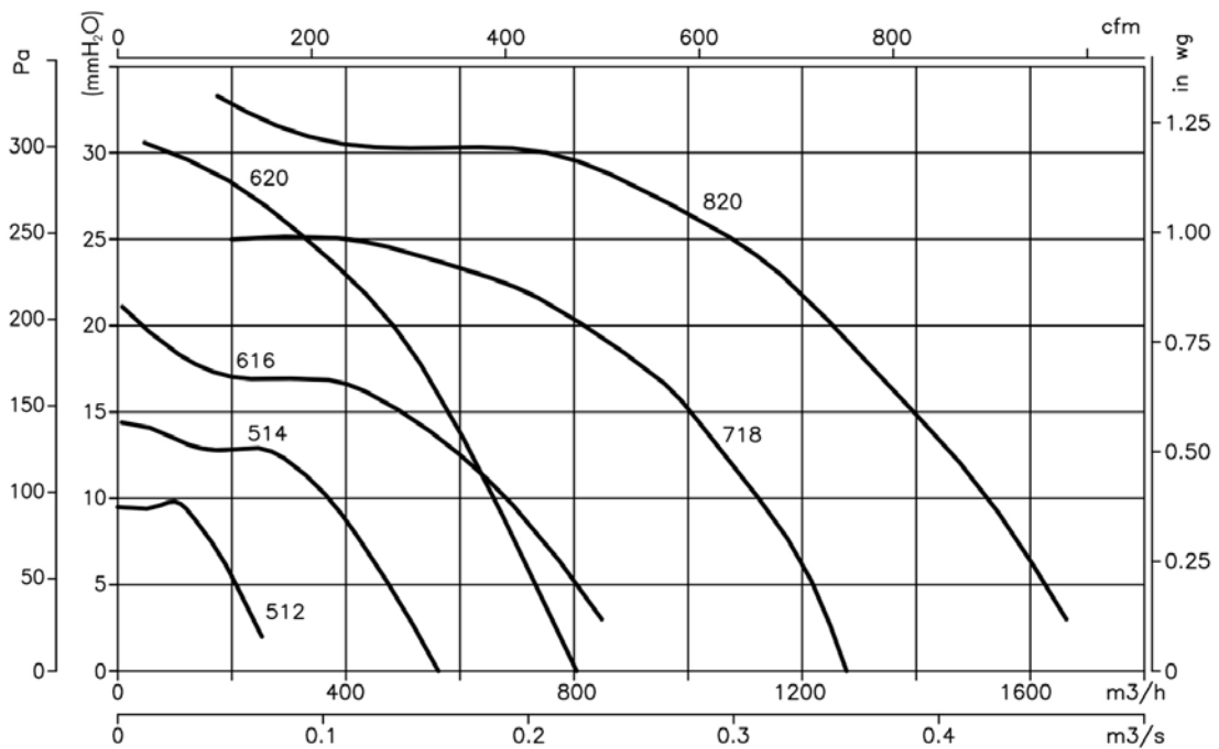
4T/4M=1800 r/min
