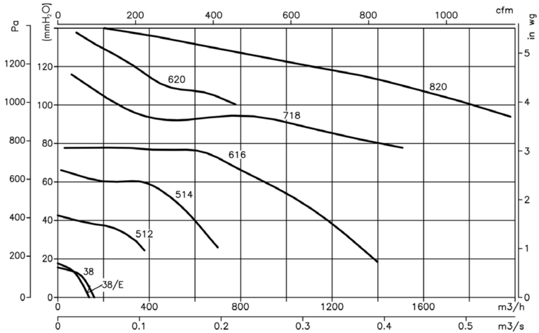
2T/2M=3600 r/min
