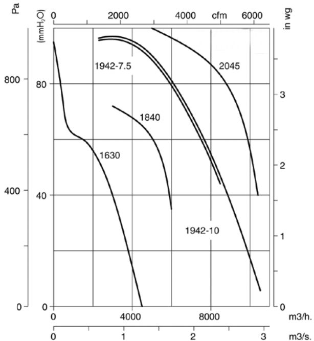
4T=1500 r/min.
