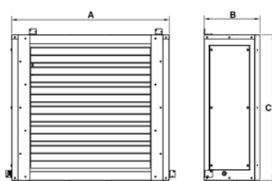
DAMPER
